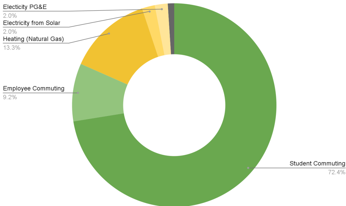
Figure 1 - GHG Emissions, 2018.
